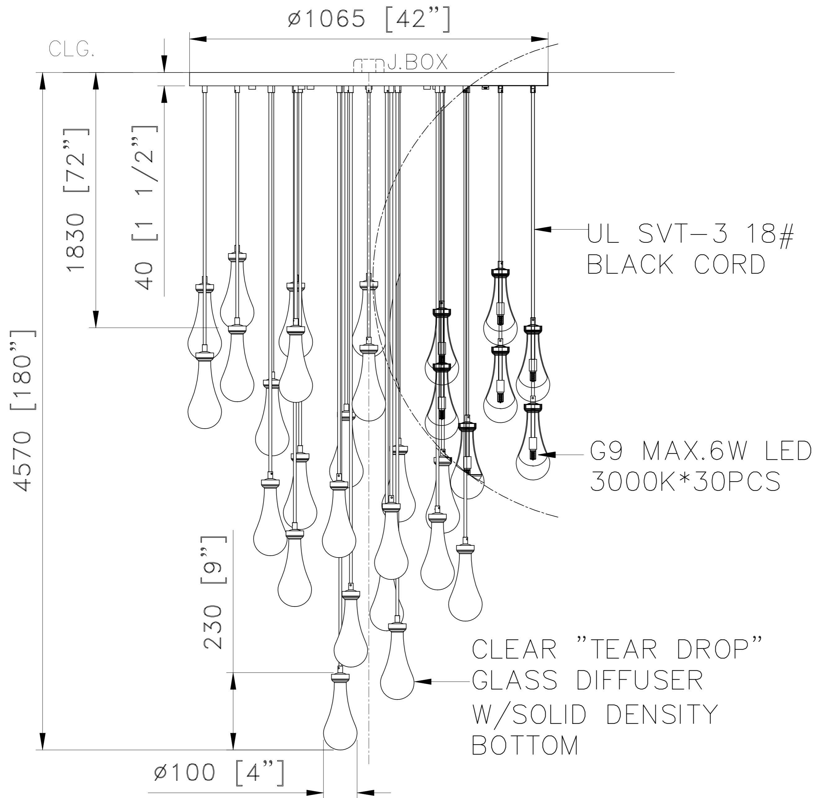
FRONT VIEW SCALE: 1 : 20
