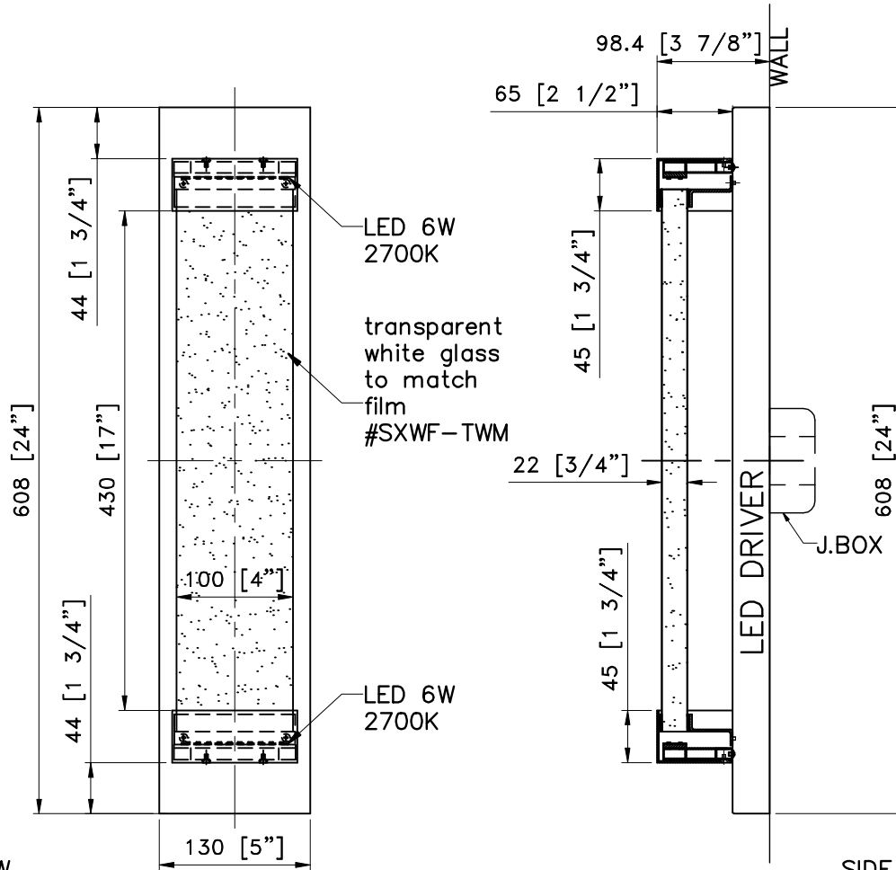
SIDE VIEW
