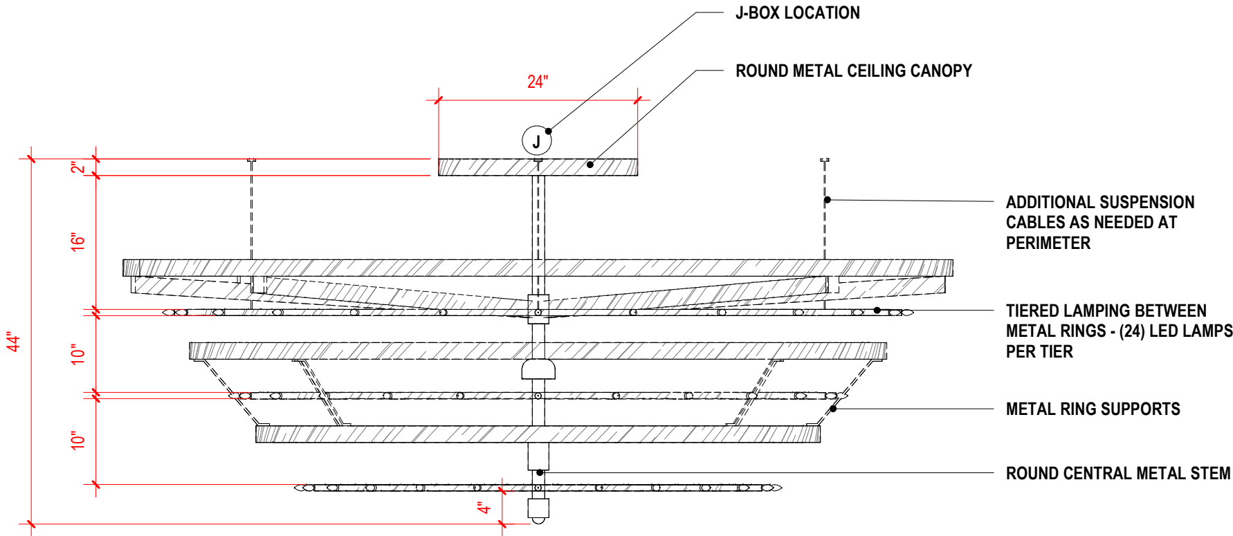
2 CHANDELIER (CH-03) INTERIOR STRUCTURE - FRONT 5401.1 SCALE: 3/4" = 1'-0"
