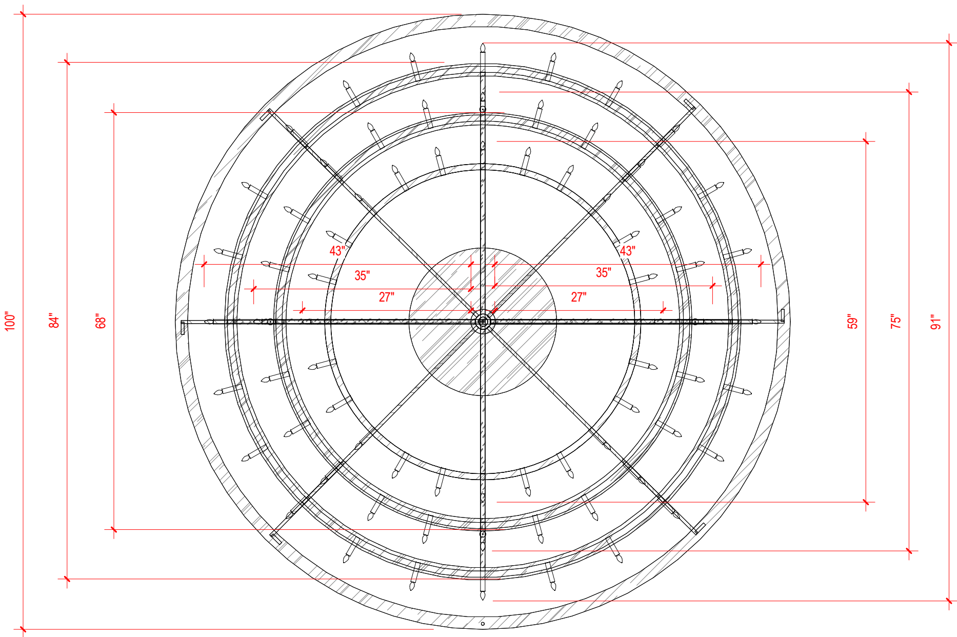
1 CHANDELIER (CH-03) INTERIOR STRUCTURE - PLAN 5401.1 SCALE: 3/4" = 1'-0"
