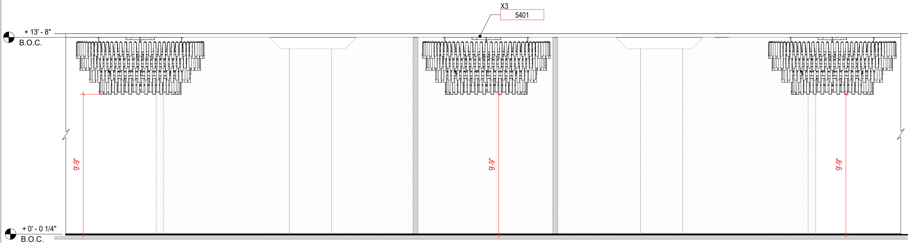
1 5401 DECORATIVE LIGHTING ELEVATION 5401 - CHANDELIER (CH-03) SCALE: 1/4" = 1'-0"
