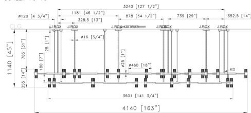
FRONT VIEW SCALE: 1 : 40
