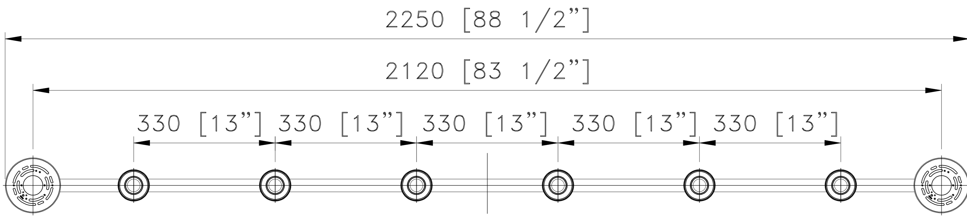
TOP VIEW
